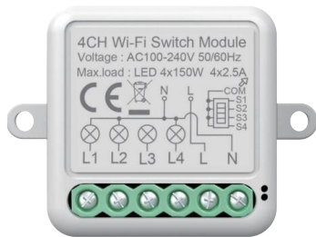
Smart Breaker (Switch/Dimmer/Curtain)
