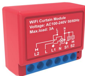
Smart Breaker (Switch/Dimmer/Curtain)
